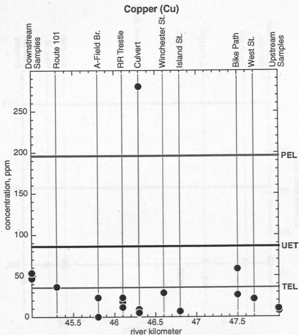
Figure 6: Results for Copper, , concentration versus river kilometer for samples in Keene (Fig. 2). Samples from downstream and upstream of Keene (Fig. 1) are also plotted, but not by river kilometer. Freshwater sediment UET, PEL and TEL values from Buchman (1999).
